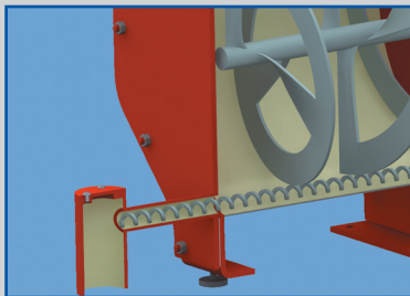
Cutaway showing spiral auger with scroll agitator
